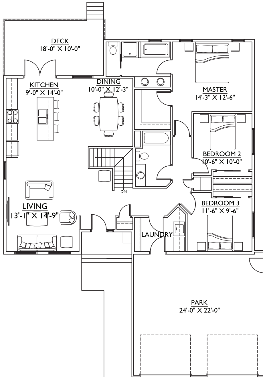
MAIN FLOOR PLAN | 1535 SQ. FT.
