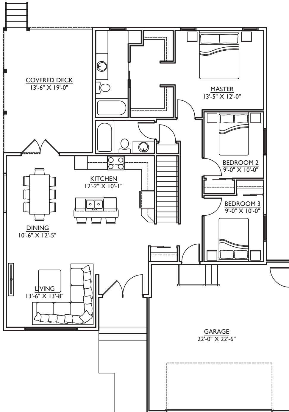
MAIN FLOOR PLAN | 1369 SQ. FT.
