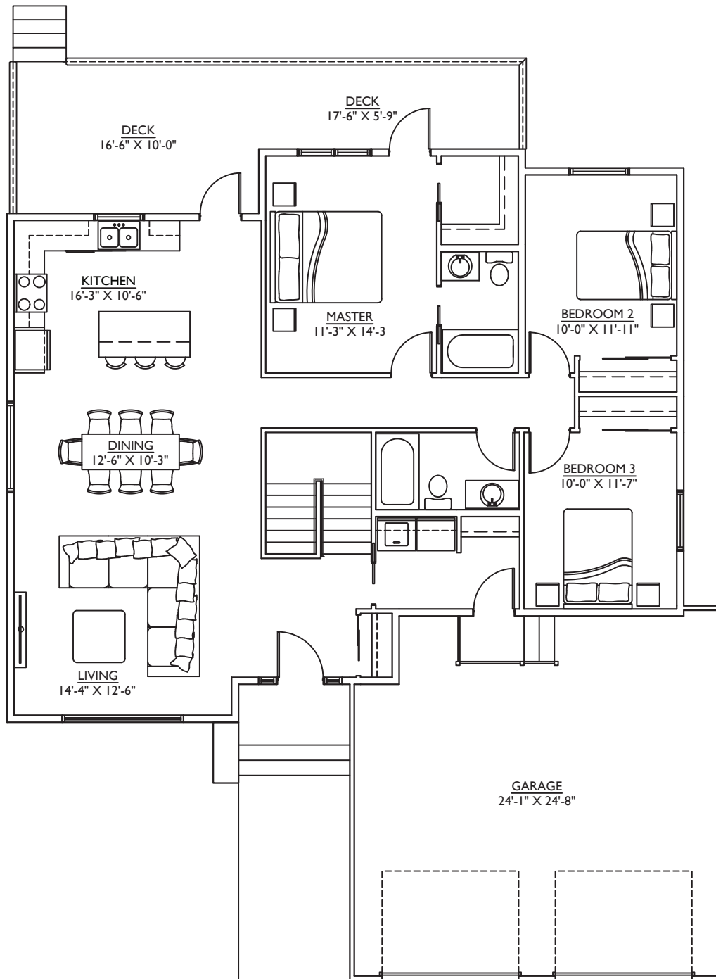
MAIN FLOOR PLAN | 1433 SQ. FT.
