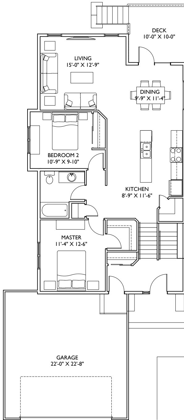
MAIN FLOOR PLAN | 1152 SQ. FT.
