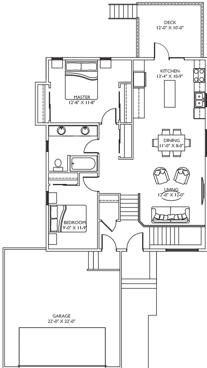
MAIN FLOOR PLAN | 1096 SQ. FT.
