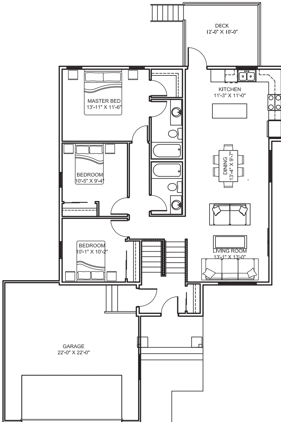
MAIN FLOOR PLAN | 1267 SQ. FT.
