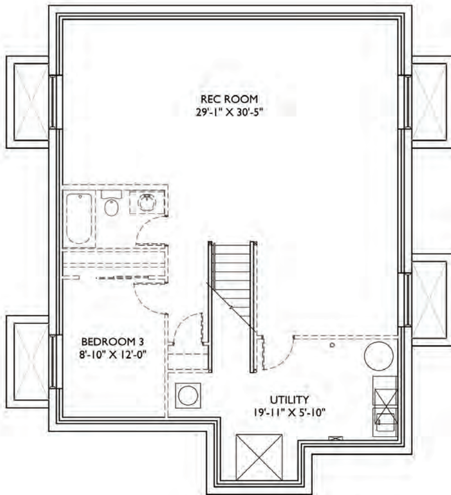
PROPOSED BASEMENT PLAN
