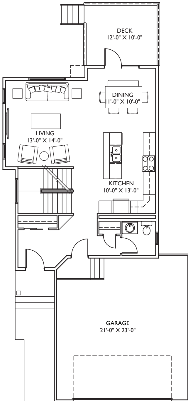
MAIN FLOOR PLAN | 1233 SQ. FT.
