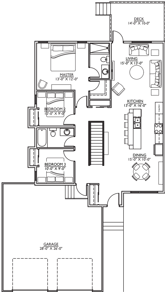
MAIN FLOOR PLAN | 1330 SQ. FT.
