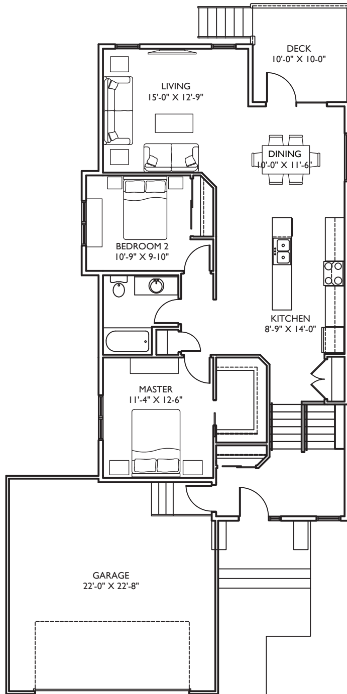
MAIN FLOOR PLAN | 1200 SQ. FT.
