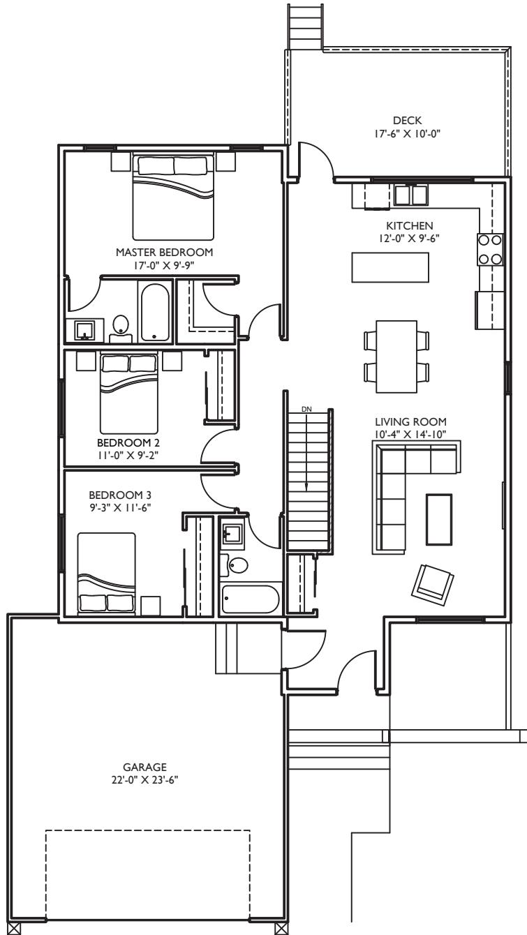
MAIN FLOOR PLAN | 1336 SQ. FT.
