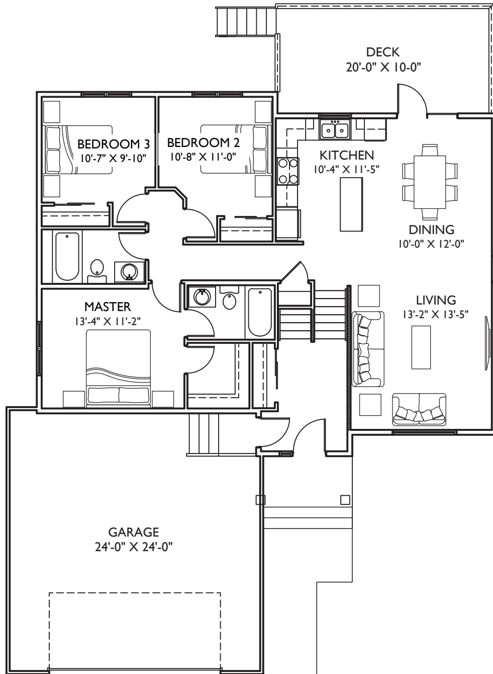
MAIN FLOOR PLAN | 1312 SQ. FT.
