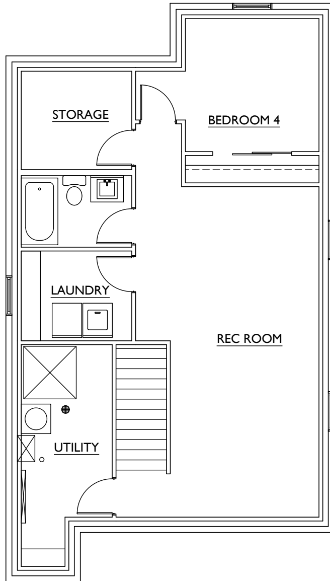
PROPOSED BASEMENT PLAN
