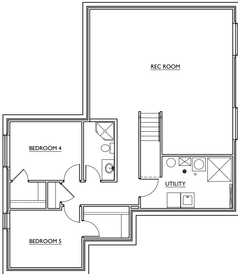
PROPOSED BASEMENT
