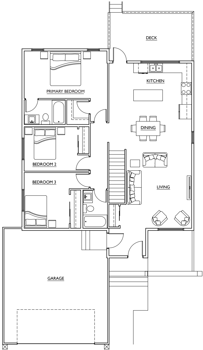
MAIN FLOOR PLAN - 1335 SQ.FT.
