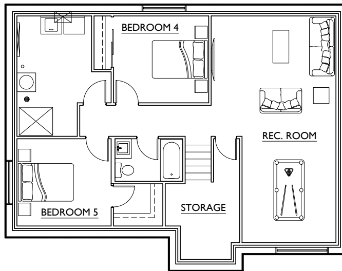
BASEMENT PLAN
