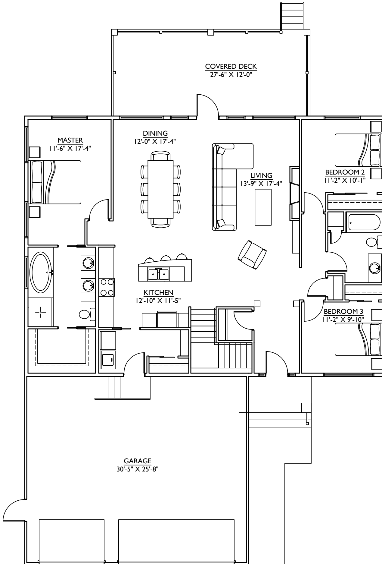
MAIN FLOOR 1800 SQ. FT.
