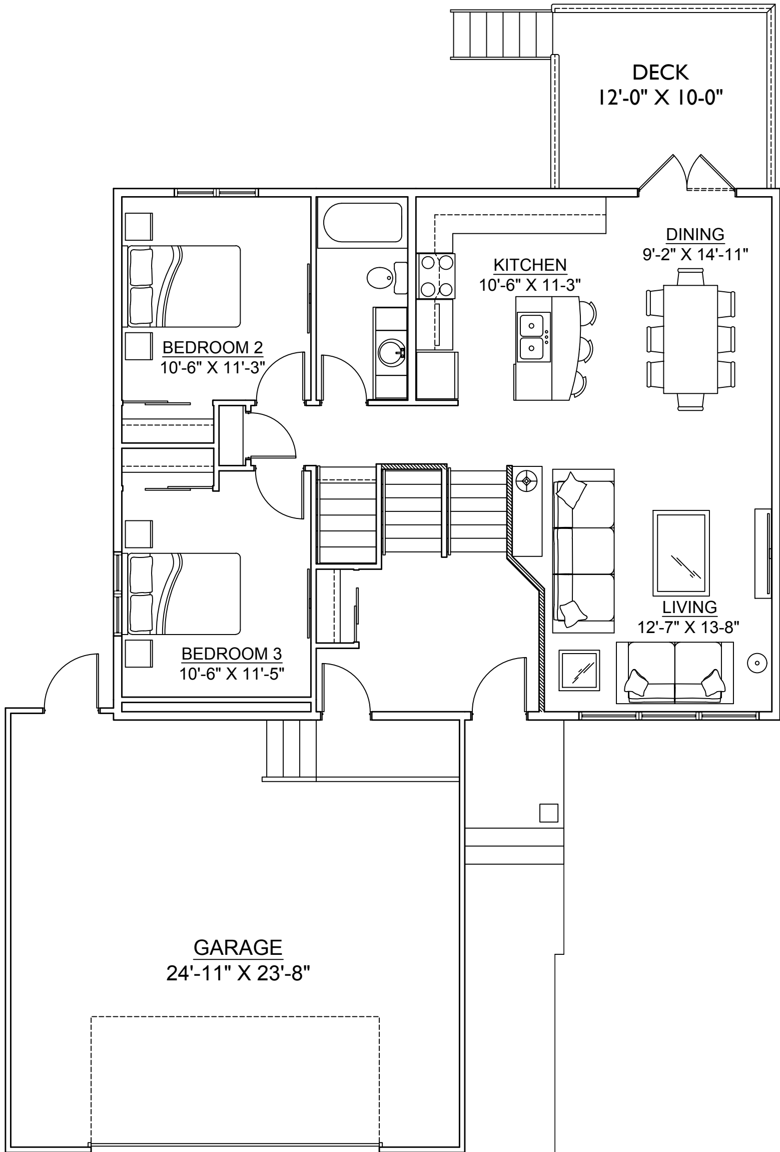
MAIN FLOOR PLAN - 1091 SQ.FT.
