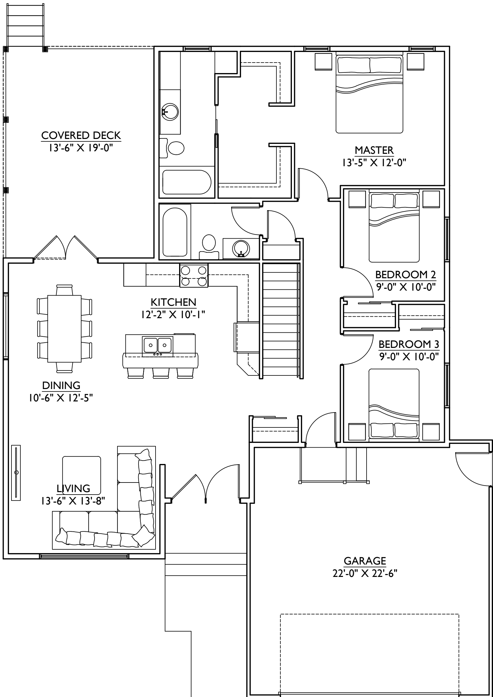
MAIN FLOOR PLAN - 1369 SQUARE FEET
