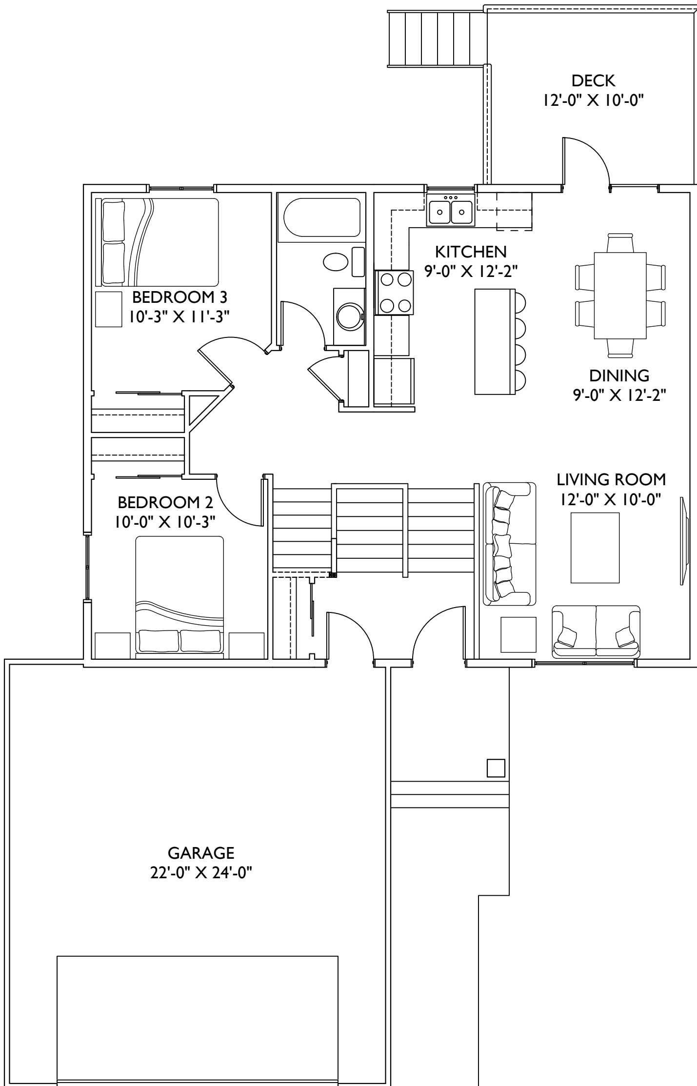
(A1) MAIN FLOOR PLAN - 963 SQ. FT. 1/4" = 1'
