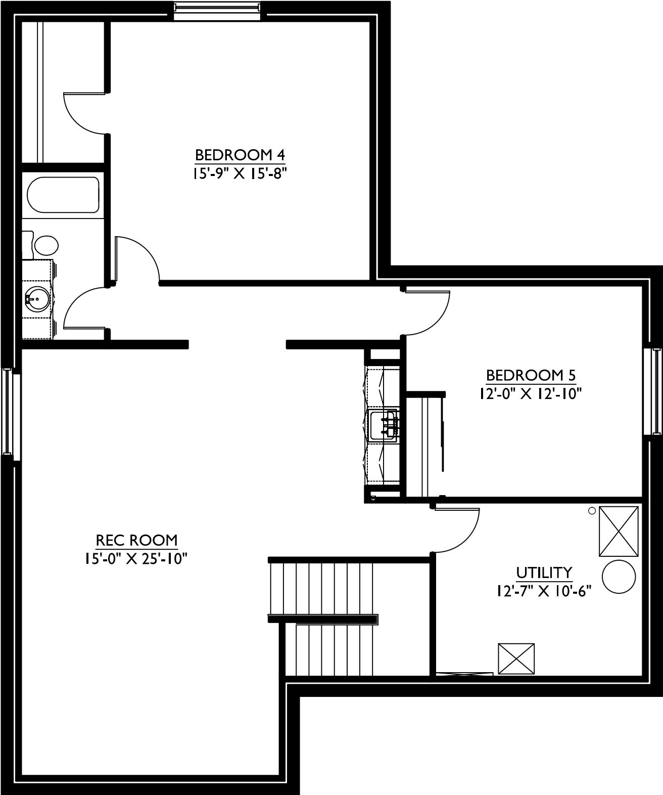
BASEMENT FLOOR PLAN - 1524 SQ. FT.
