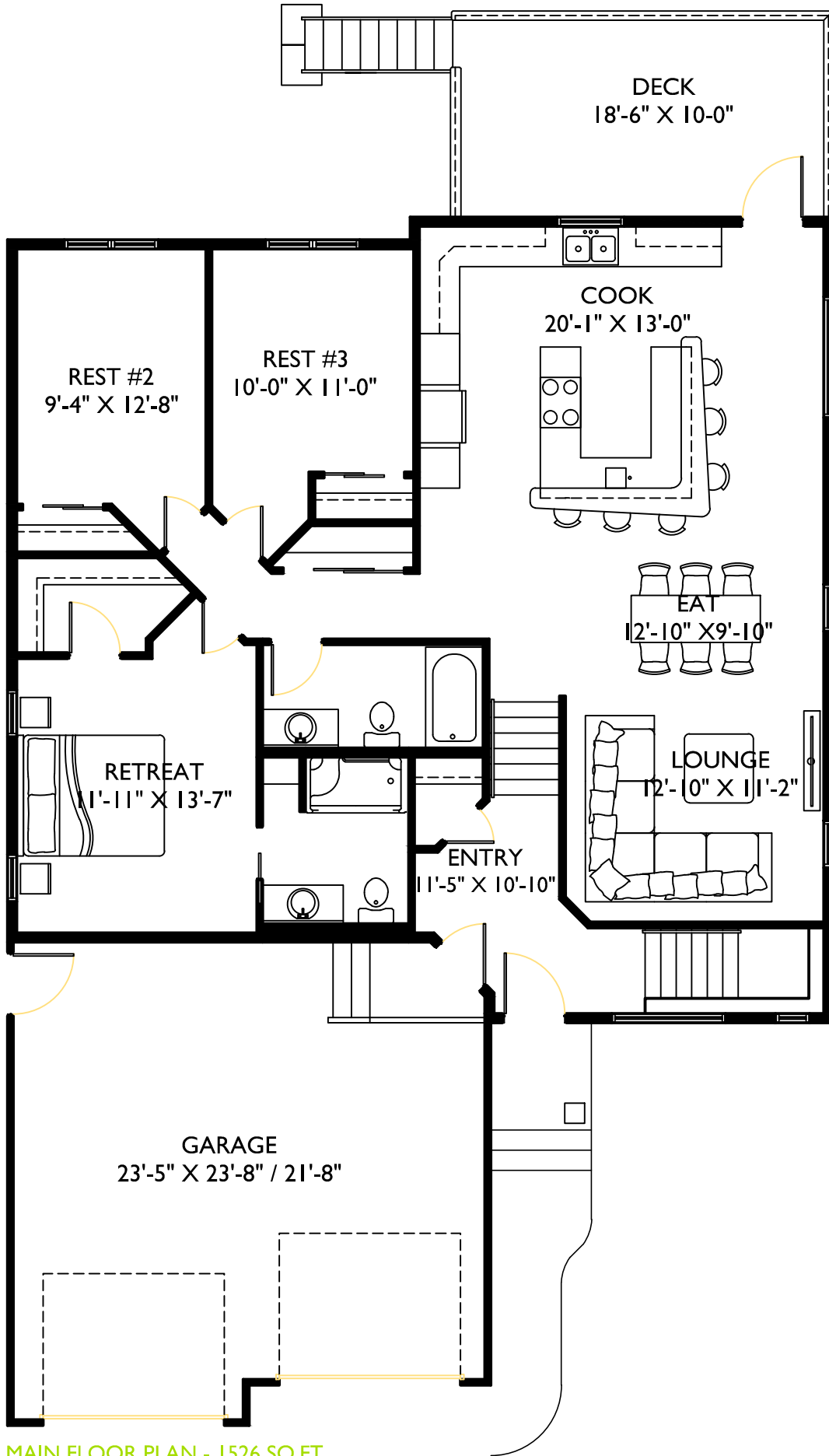
MAIN FLOOR PLAN - 1526 SQ.FT.
