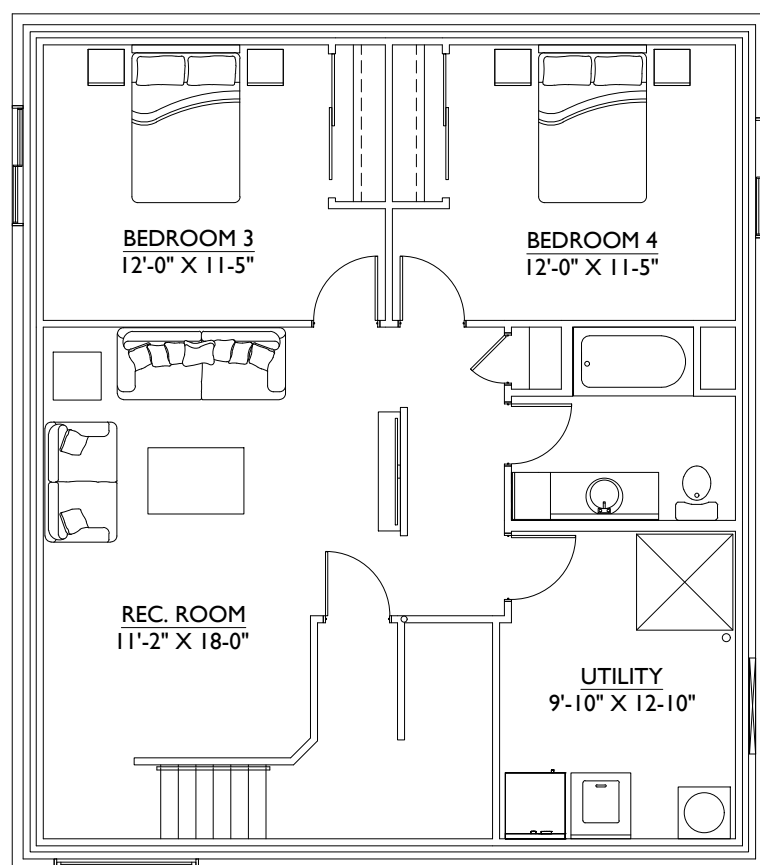
FUTURE BASEMENT PLAN 1120 SF
