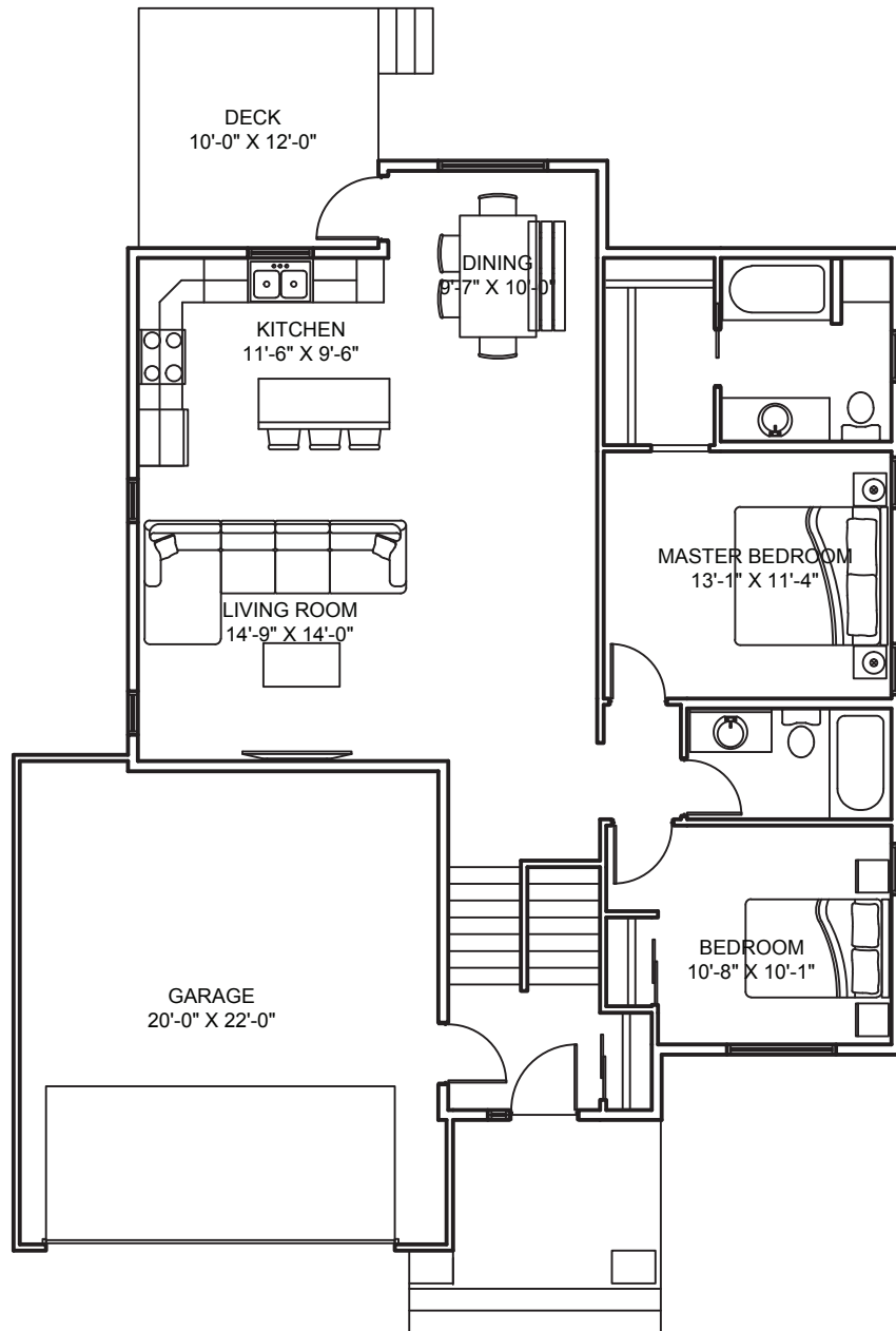
MAIN FLOOR PLAN | 1201 SQ. FT.
