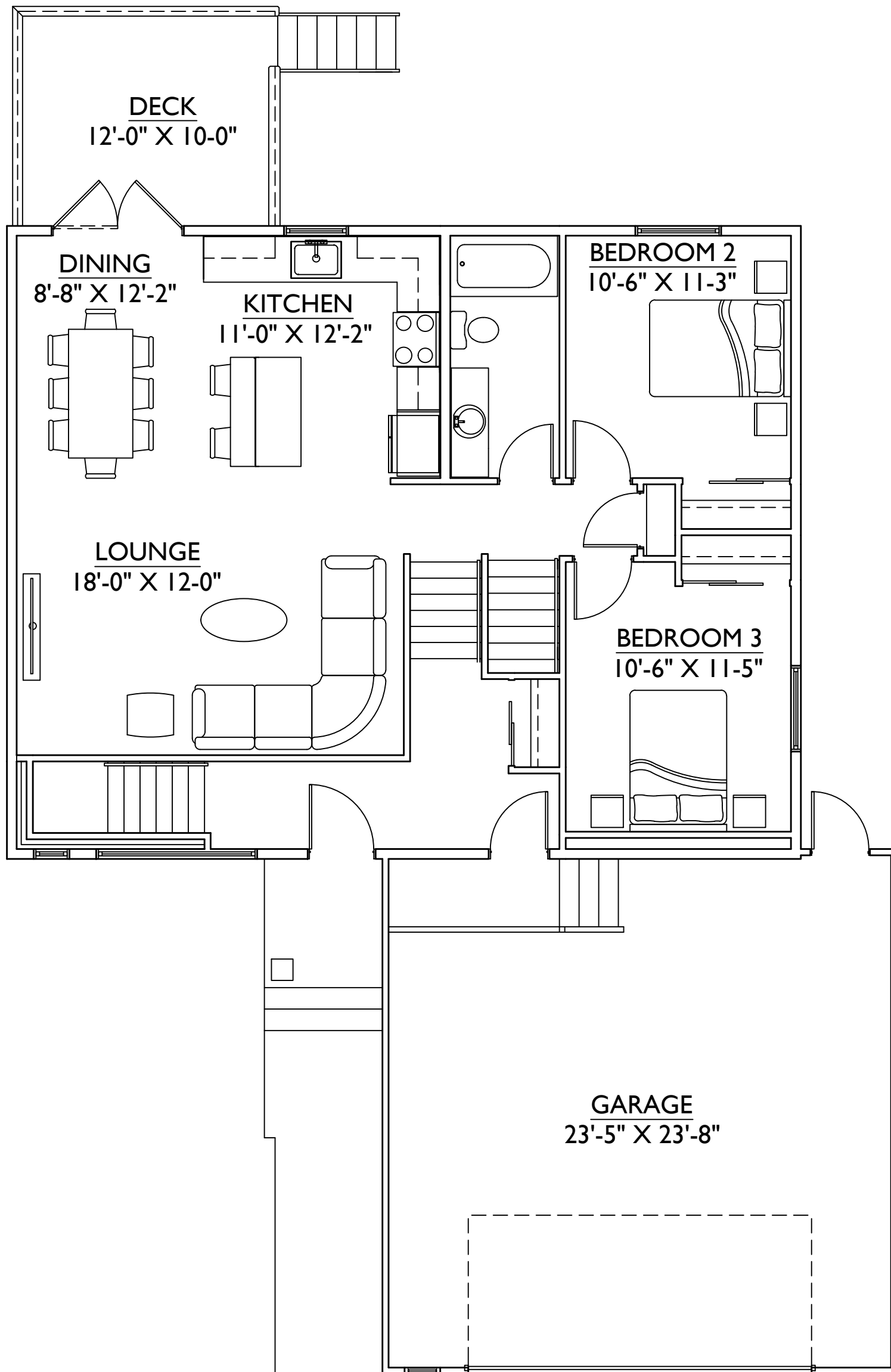
MAIN FLOOR PLAN - 1091 SQ.FT.
