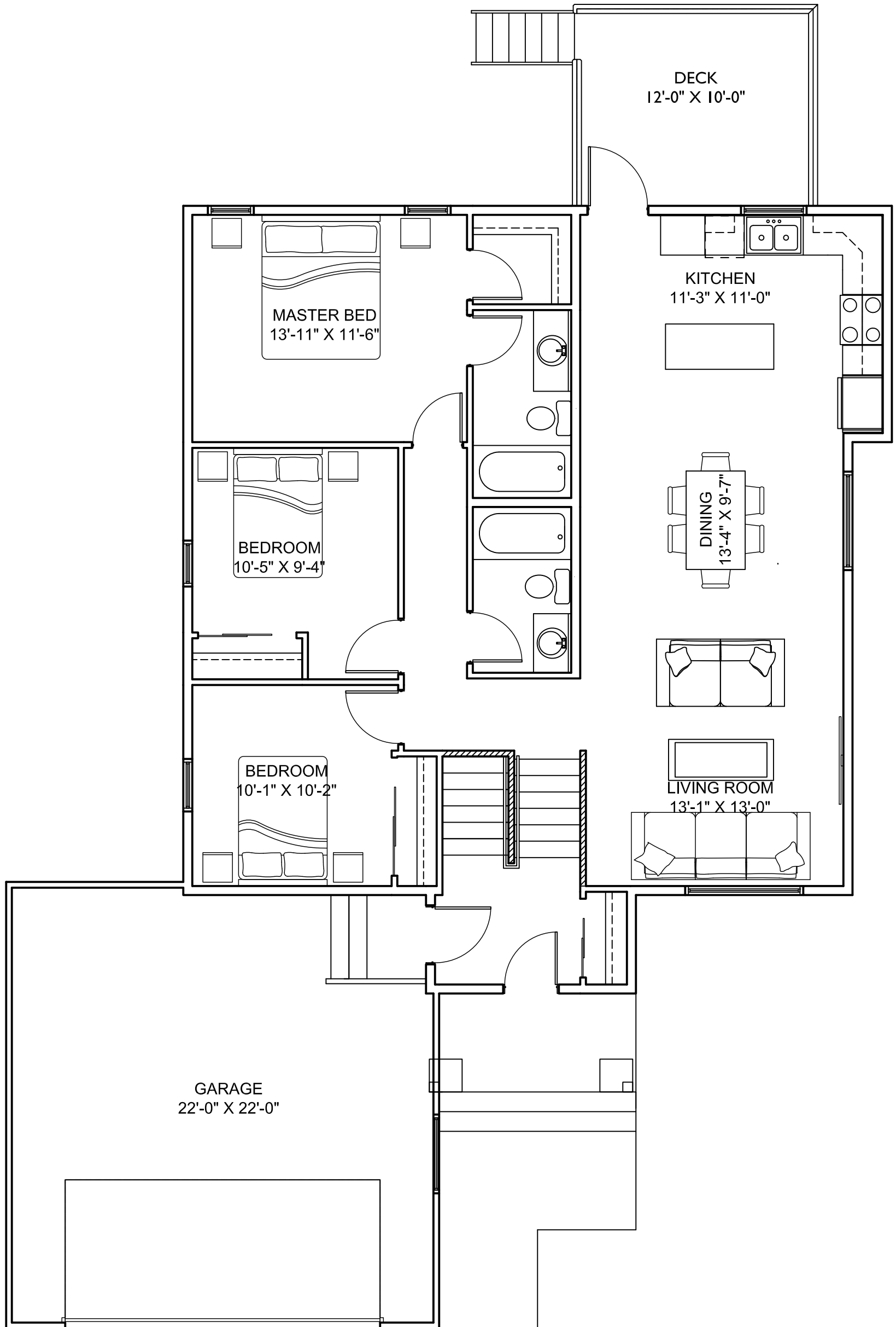
AI MAIN FLOOR PLAN - 1267 SQ.FT. 3/16" = 1'
