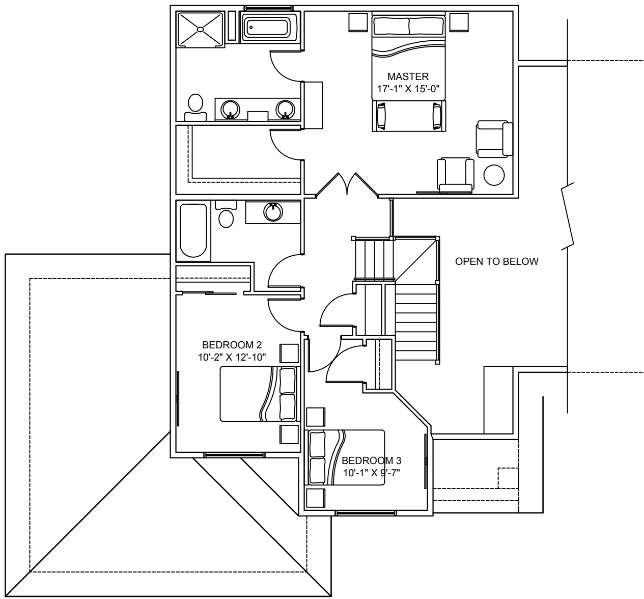
SECOND FLOOR PLAN - 893 SQ.FT.
