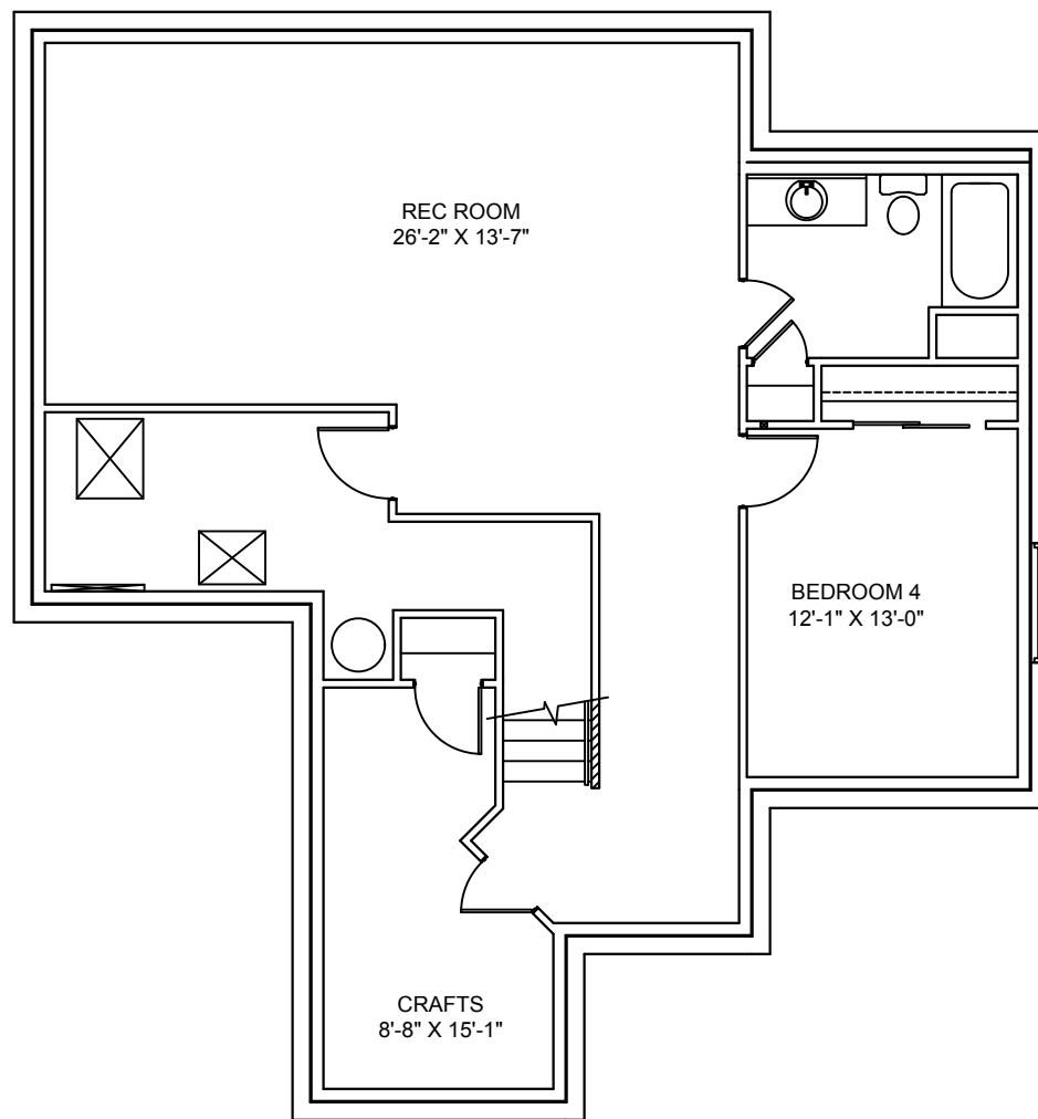
FUTURE BASEMENT PLAN
