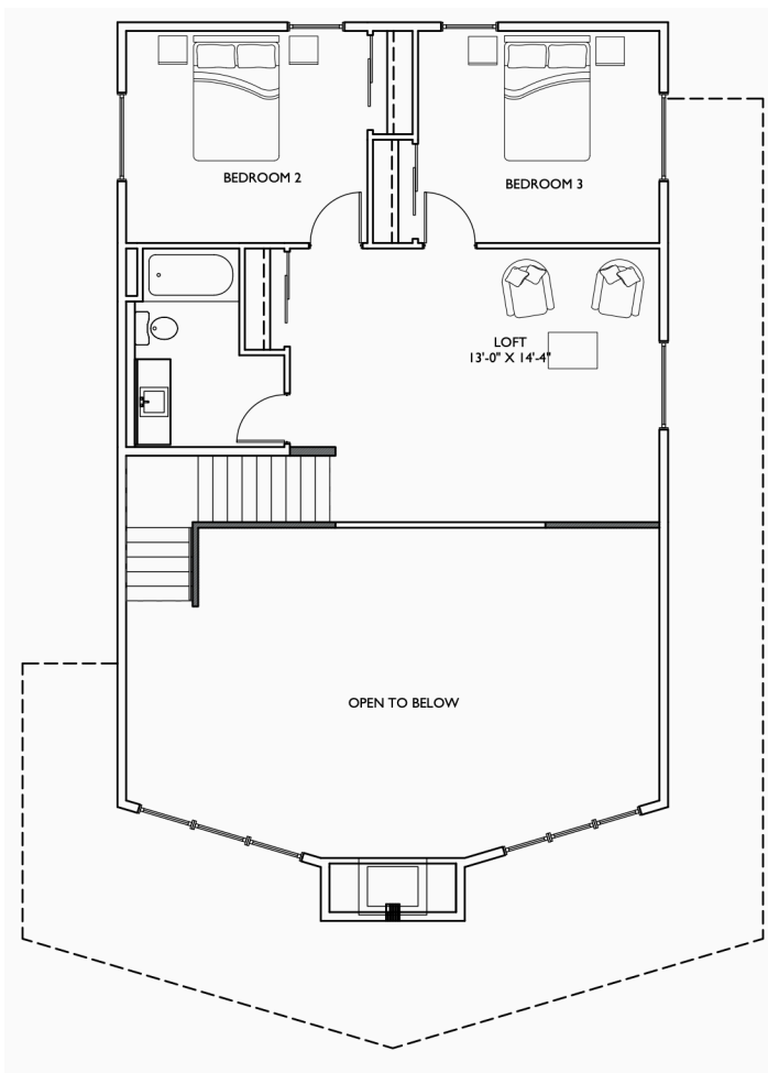
LOFT FLOOR PLAN
