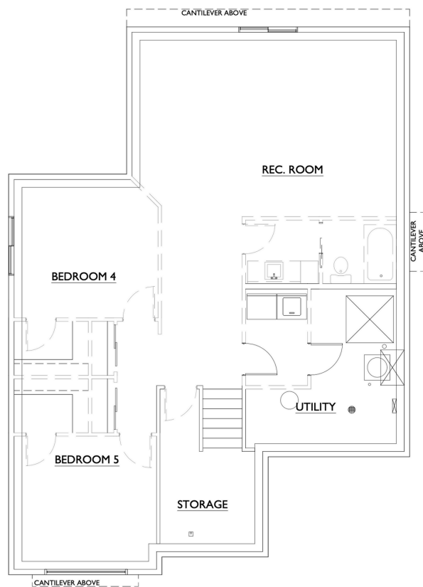
PROPOSED BASEMENT PLAN
