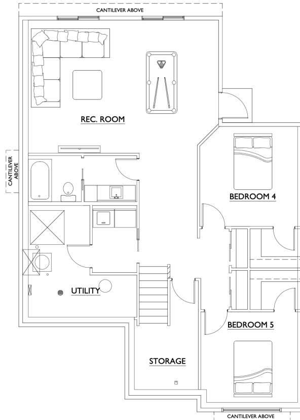
BASEMENT PLAN
