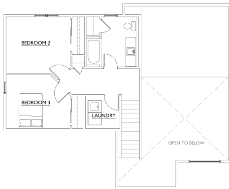
SECOND FLOOR PLAN - 548 SQ.FT.
